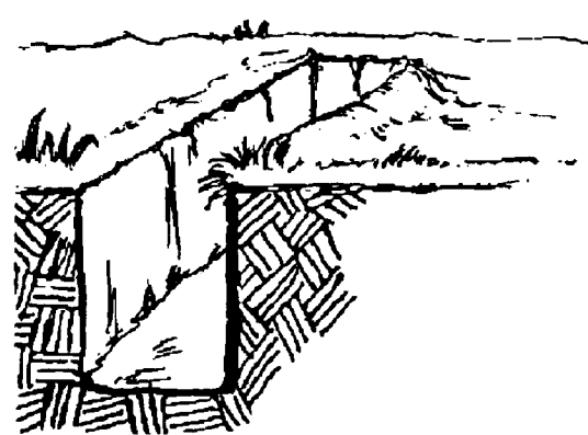
OPEN ONE-PERSON FOXHOLE
